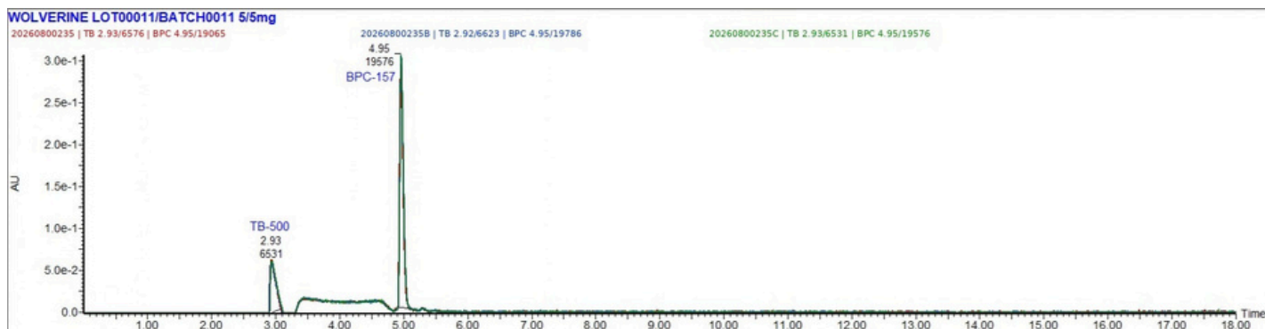
UV CHROMATOGRAM
