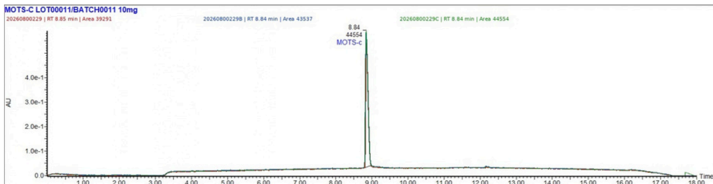
UV CHROMATOGRAM
